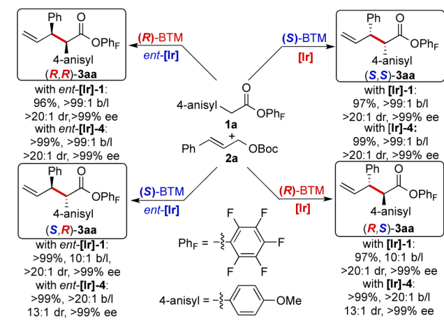
Scheme 2. Synthesis of All Four Stereoisomers of 3aa
