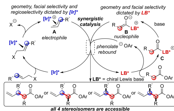
Scheme 1. Proposed Mechanism for Synergistic Catalysis
